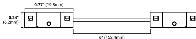
Uni-CCT-3P-TT-6W-12 (Tape-to-tape snap connector with 6" wire)
