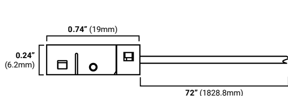
Uni-CCT-3P-TW-72W-12 (Tape to wire snap connector with 72" wire)
